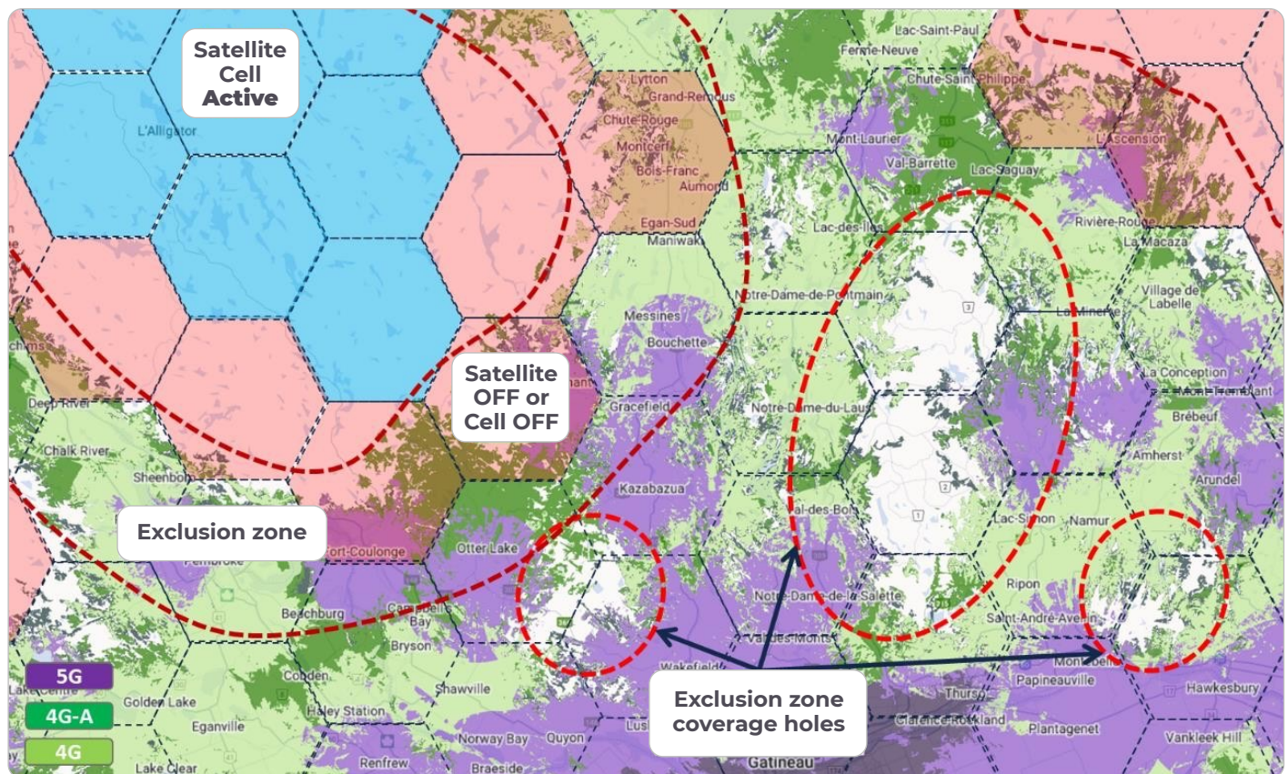
Figure 3: Typical D2D spectrum sharing deployment scenarios with service exclusion zones
